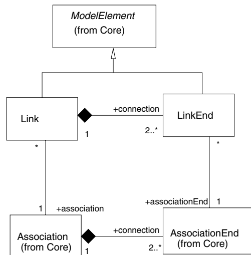
Fig. 7. Extract from UML1.4 metamodel
