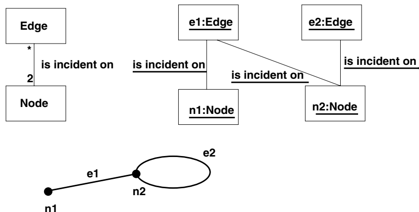
Fig. 3. An incorrect way to use UML1.4 multiplicities
